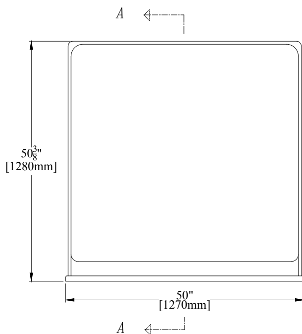
50" [1270mm] Dome for Model 5050BF
