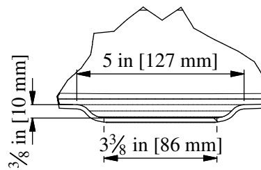
DETAIL C@ Drain
