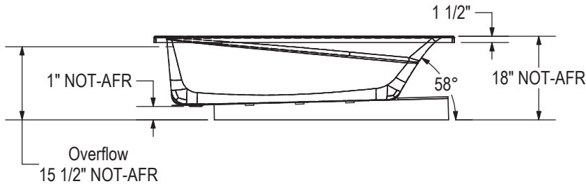
WHIRLPOOL SYSTEM
